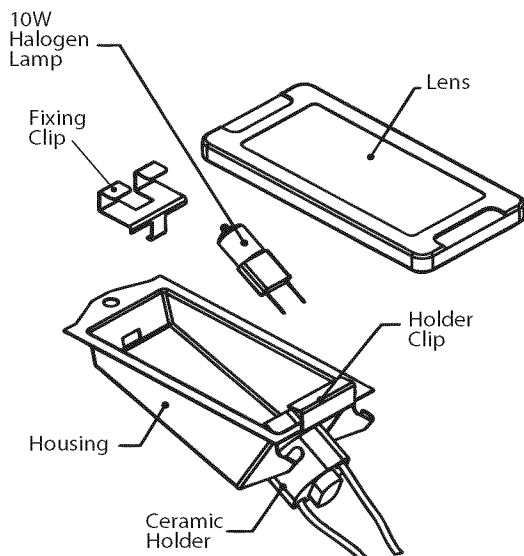
Figure 33: Oven Lamp Assembly
